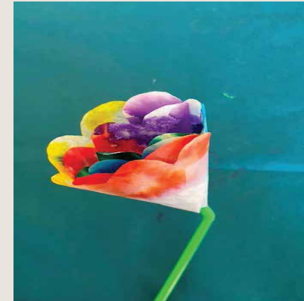
CHROMATOGRAPHY
